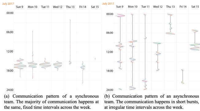
Figure 2: Visualization of the communication pattern between synchronous collaboration and asynchronous collaboration style [11]. Each line indicates a conversation thread in the team. The Y-axis denotes the time of the day. The amplitude along X-axis denotes conversation intensity at that time frame.
