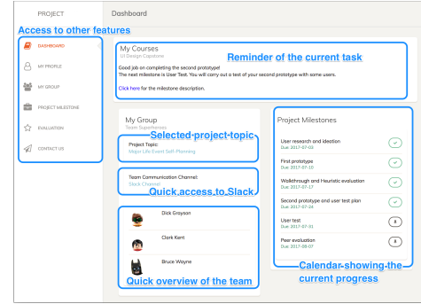
Figure 1: The homepage of ProjectLens, which can be directly integrated with major MOOC platforms
